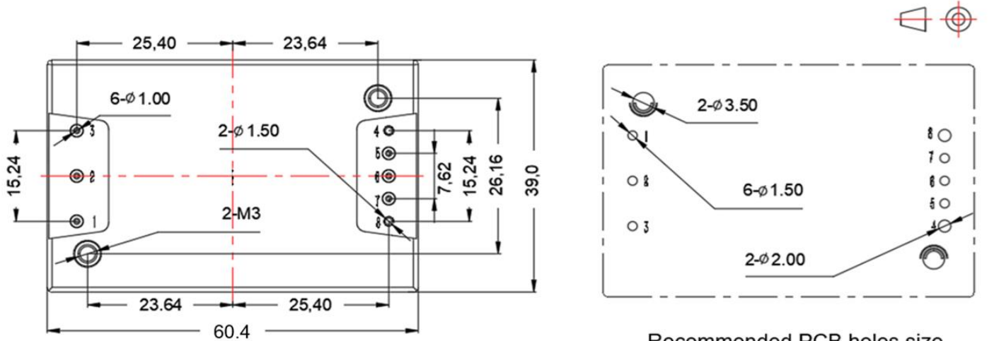
Recommended PCB holes size
