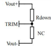
Voltage-down: Add R_{down} between Trim and Vout+
