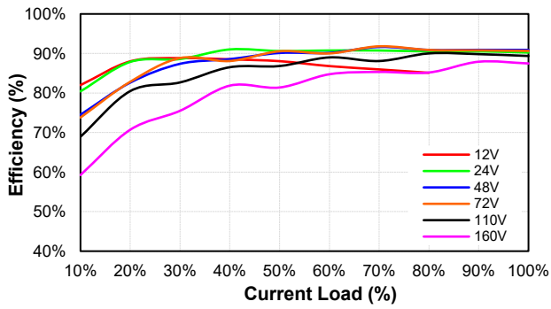
CQB100W14-72S54 Eff Vs Io @25 Deg. C
