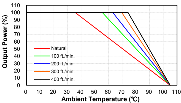
CQB100W14-72S15, 24, 28, 54 Derating Curve with Heatsink QBL127 (Vin=72V)
