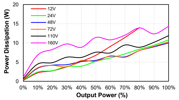
CQB100W14-72S54 Pd Vs Po @25 Deg. C
