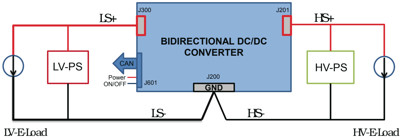
Fig. 2: The bench setup used to operate 48S12.3K0BCA and take measurements provided in data sheet. The combination of the Electronic Load (E-Load) and Bench Power Supply (PS) emulates a battery capable of both sourcing and sinking current.
