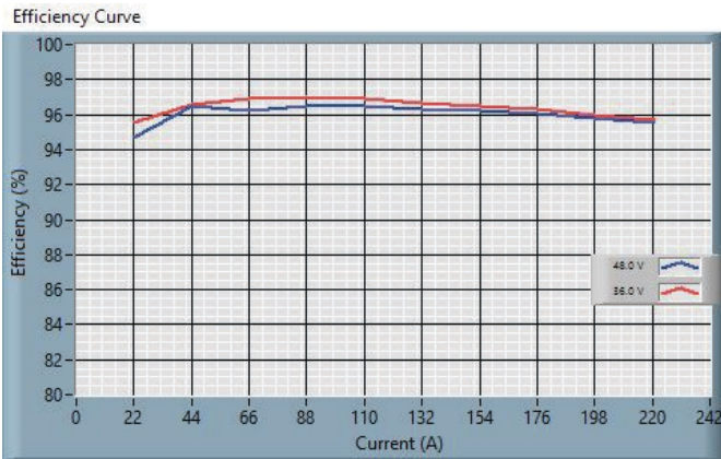
Fig. 1: 48S12.3K0BCA Efficiency Curve – Buck Mode, V_o=14V .
