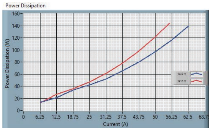
Fig. 4: 48S12.3K0BCA Power Dissipation – Boost Mode V_o=48V
