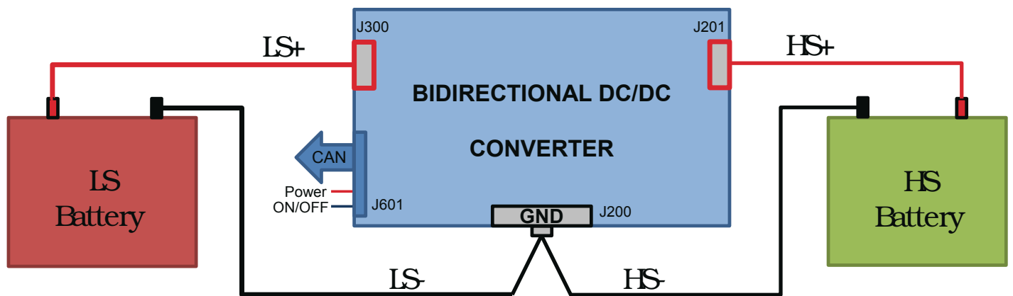
The 48S12.3K0BCA block diagram.
