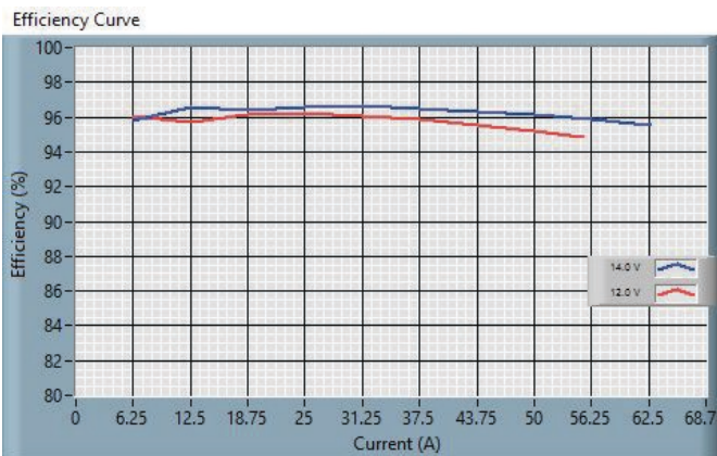
Fig. 3: 48S12.3K0BCA Efficiency Curve – Boost Mode, V_o=48V
