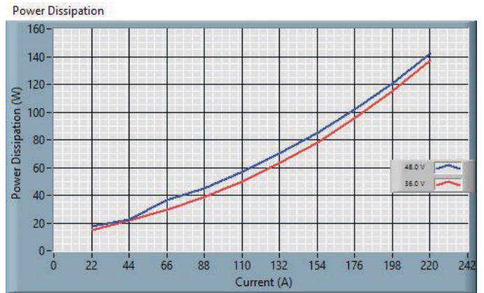
Fig. 2: 48S12.3K0BCA Power Dissipation – Buck Mode, V_o=14V .
