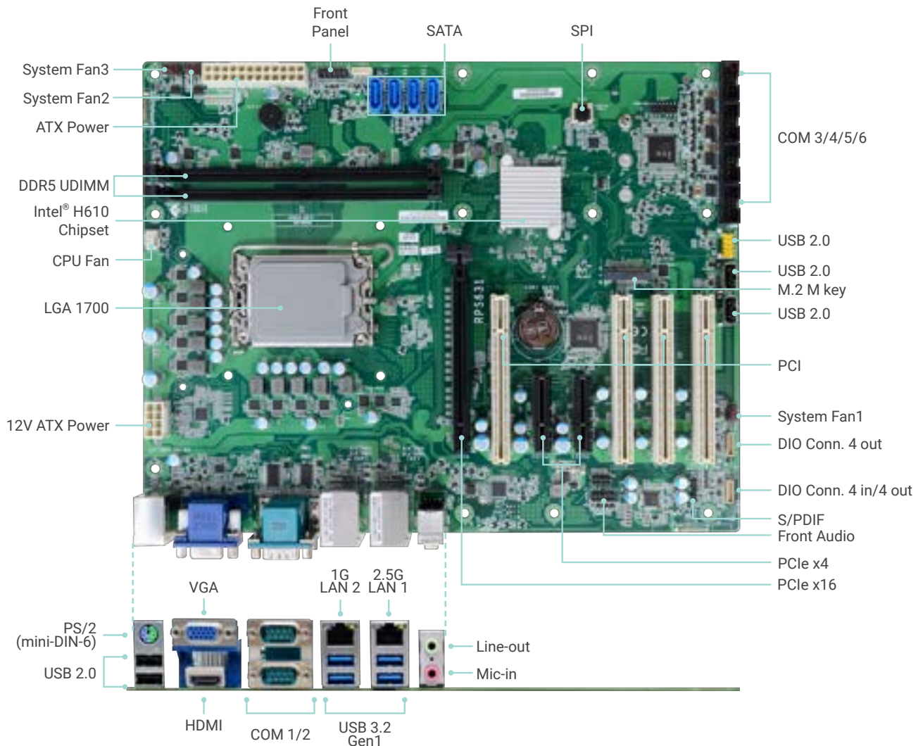
Top View
