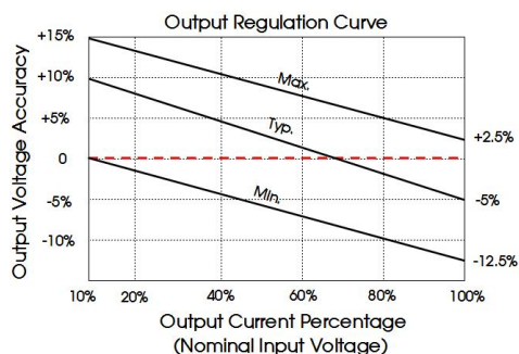
3.3VDC output
