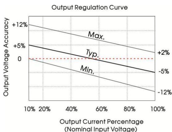
Fig. 1(3.3VDC output)
