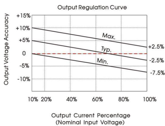
Fig. 1(Others output)
