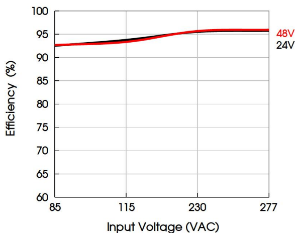
Input Voltage Vs Efficiency (Full Load)
