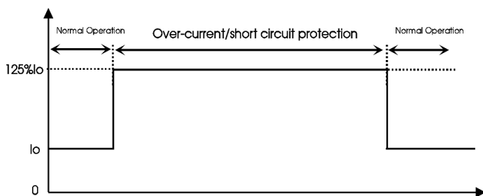
Over-current/ Short circuit protection curve (Typ.)
