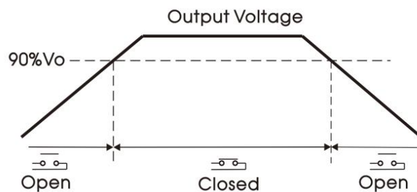
DC OK behavior curve (Typ.)
