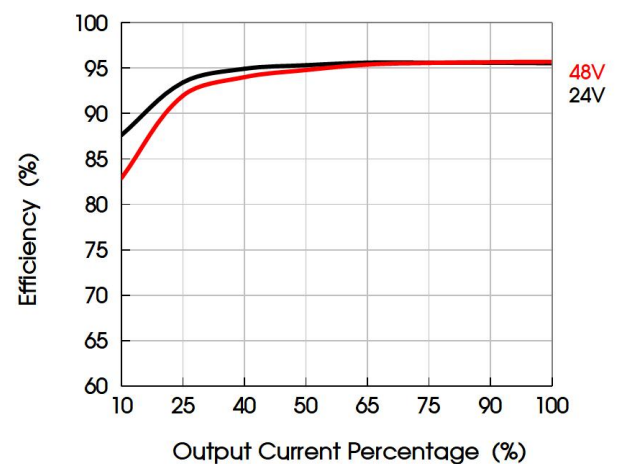
Output Load Vs Efficiency (Vin=230VAC)
