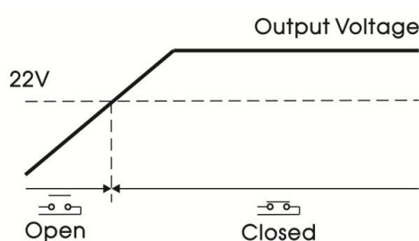
DC OK behavior curve (Typ.)
