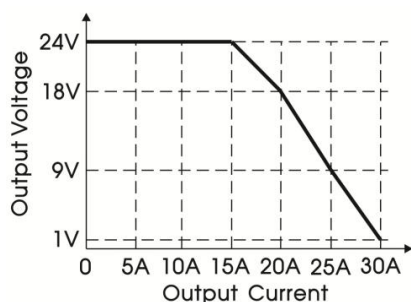
Over-current protection curve (Typ.)
