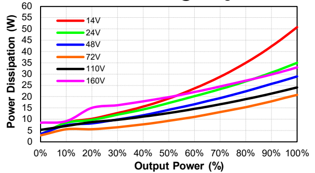
CHB200W12-72S12-CMFD Pd Vs Po @25 Deg. C
