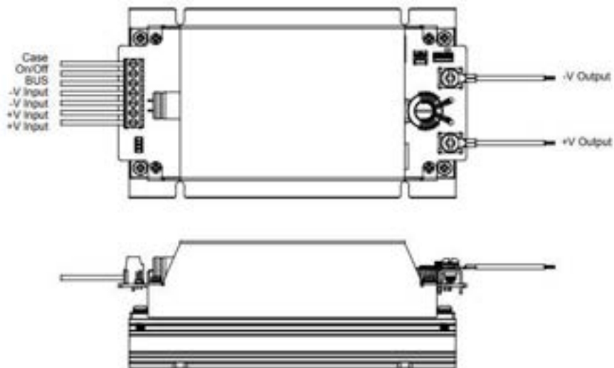
Figures 2 CHB200W12-72SXX-CMFD with Heat Sink CMLH02
