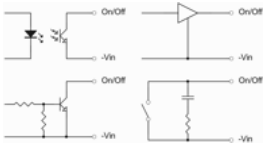
Remote On/Off Connection Example
