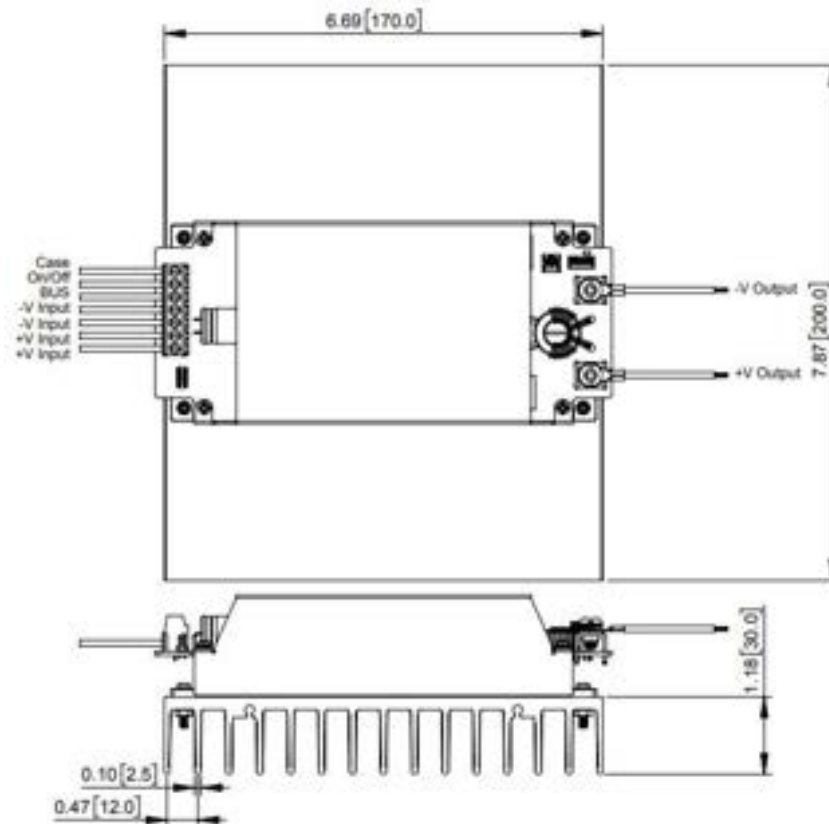
Figures 1 CHB200W12-72SXX-CMFD with Heat Sink (7.87x6.7x1.18inch)
