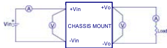
CHB200W12-72SXX-CMFD Series Test Setup
