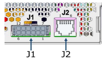
Signal and Communication Connector (J1 & J2)
