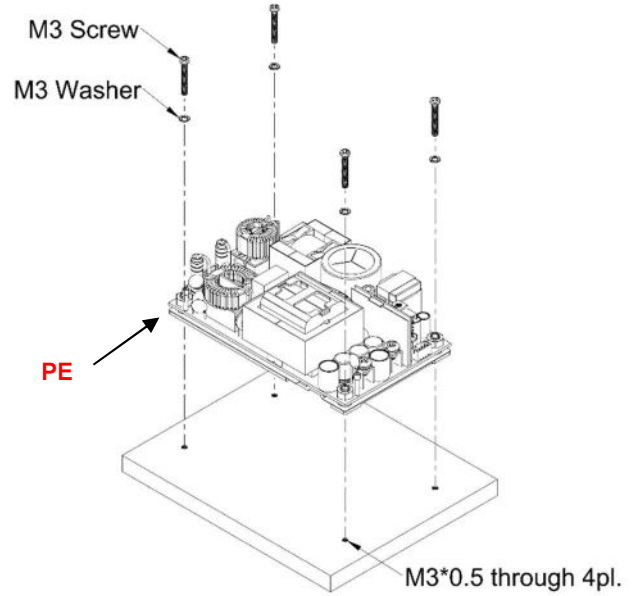
CFM400SXXXC installation diagram
