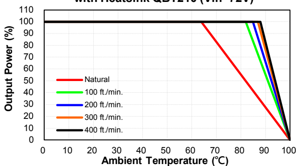
CQB50W12-72S Derating Curve with Heatsink QBT210 (Vin=72V)
