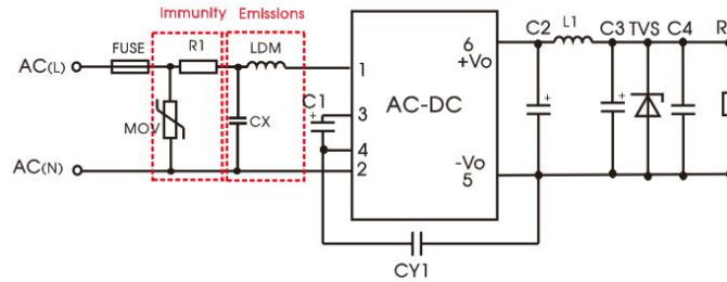
Application circuit 3
