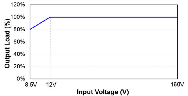
EC7AW18-72 Input Voltage Derating Curve
