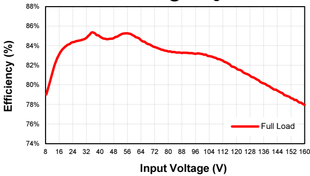
EC7AW18-72S05 Eff Vs Io @25 Deg. C
