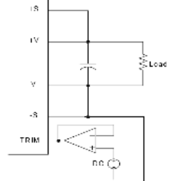
Figure 2 The schematic of output voltage adjusted by using external DC voltage.
