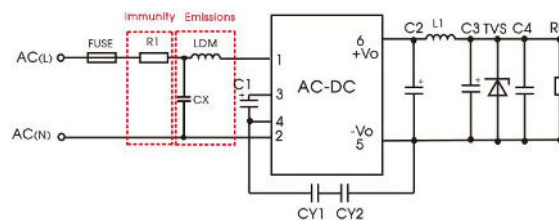
Recommended circuit 2
