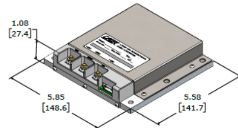
ISOMETRIC VIEW (REFERENCE)
