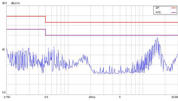
CHB300-300S48-CMFC Line
