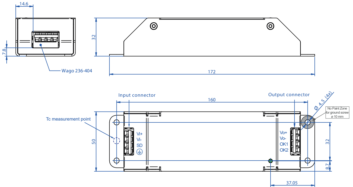
Fig. 10 Case of RCM60 with standard cage clamp terminals, Aluminum, EP-powder coated Weight approx. 350 g
