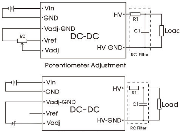
External control voltage regulation Fig.3
