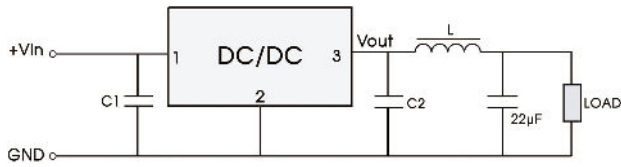
Positive output
