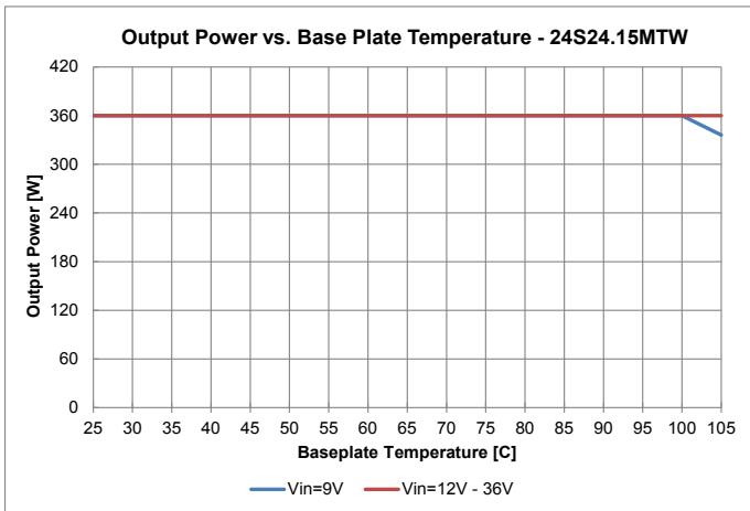
Fig. 12: 24S24.15MTW (ROHS) Derating Curve
