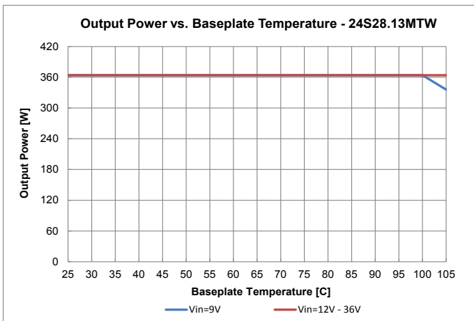
Fig. 14: 24S28.13MTW (ROHS) Derating Curve
