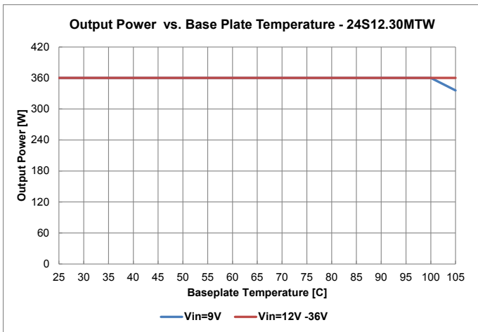
Fig. 10: 24S12.30MTW (ROHS) Derating Curve
