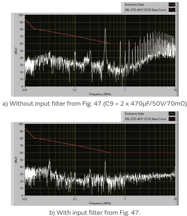
Fig. 58: Input conducted emissions measurement (Typ.) of 24S24.42FXW.
