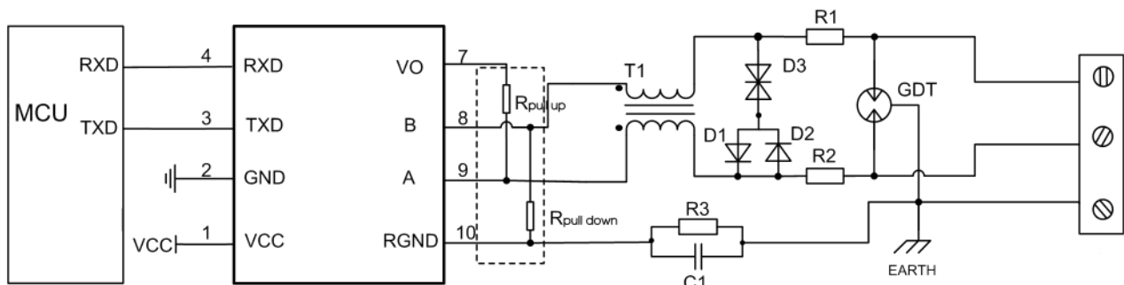
Fig.2: Port protection circuit for harsh environments
