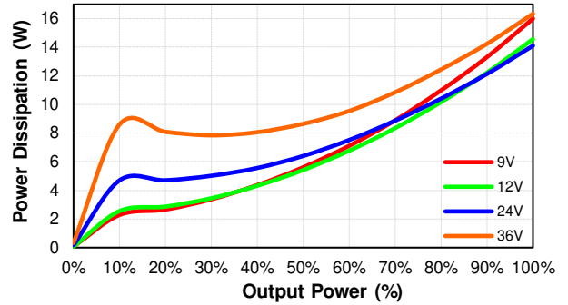
CQB150W-24S12 Pd Vs Po @25 Deg. C
