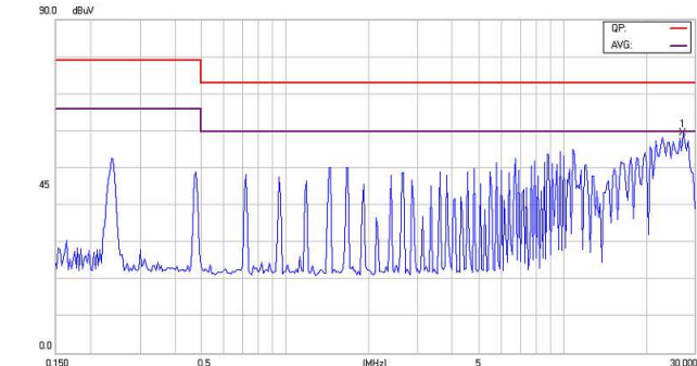
Conducted Class A of CHB200W-48S15
