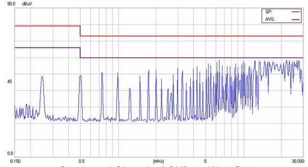
Conducted Class A of CHB200W-48S24
