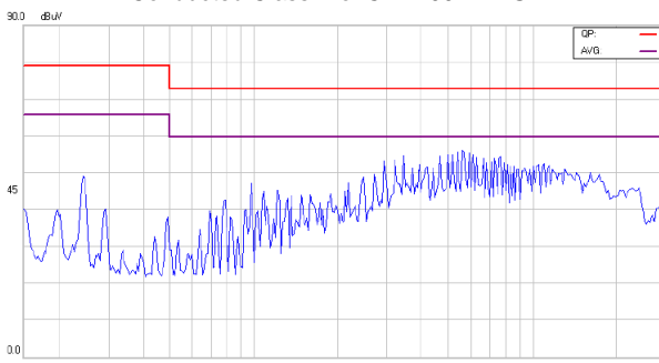
Conducted Class A of CHB200W-24S48
