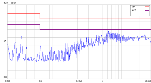
Conducted Class A of CHB200W-48S48
