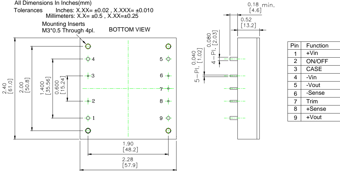
CHB200W Mechanical Outline Diagram
