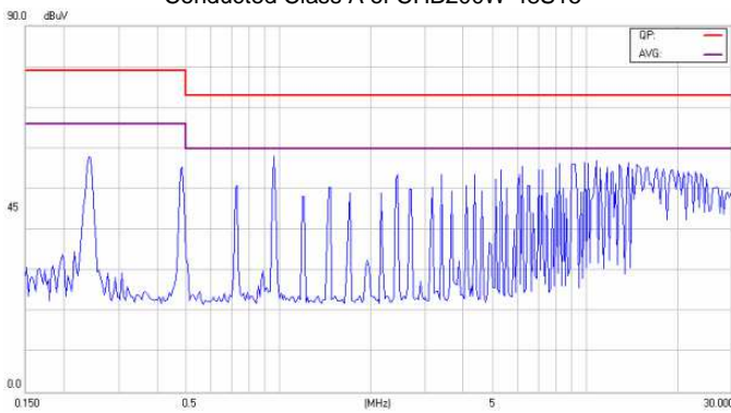
Conducted Class A of CHB200W-48S28
