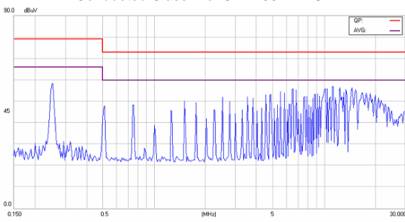
Conducted Class A of CHB200W-24S24
