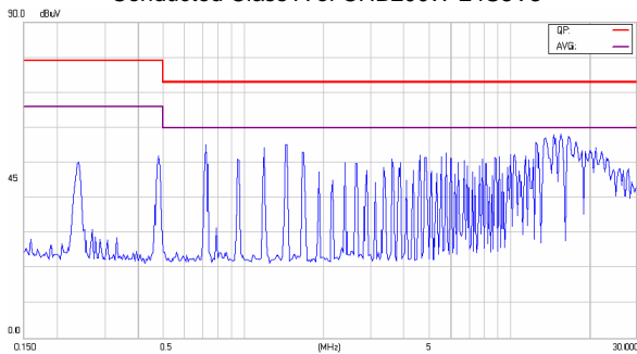
Conducted Class A of CHB200W-24S12
